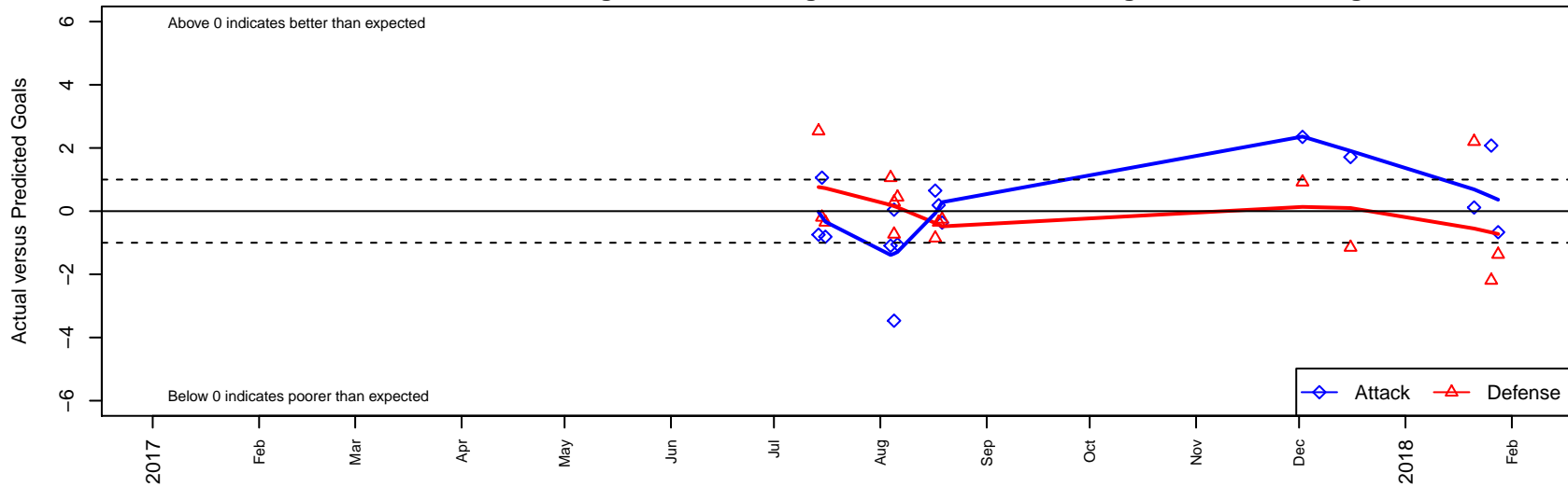
GS Surf C G03 Dots are actual minus expected GF (blue circles) and GA (red triangles). Blue line is smoothed change in attack strength. Red is smoothed change in defense strength.
